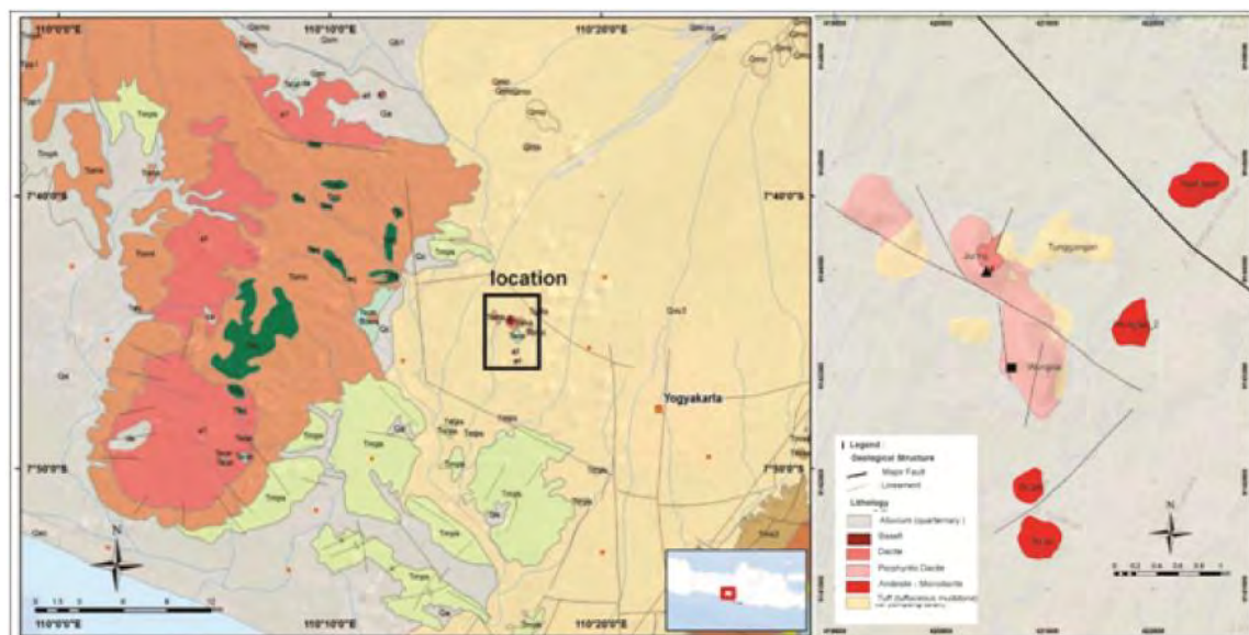
Figure 1: Location of Godean, in Regional Geology Map by Raharjo, et al. (1997) and Local Geological Map of Godean by Verdiansyah (2016a) and Location of Sample that Discuss in this Paper (Triangular Shape is for Basalt, Square Shape is for Dacite)
