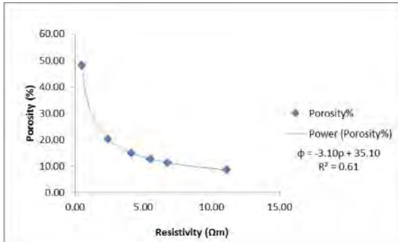
Figure 5: Porosity Against Resistivity of the Aquifer
