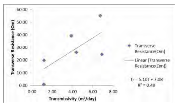
Figure 9: Transverse Resistance Against Transmissivity of the Aquifer
