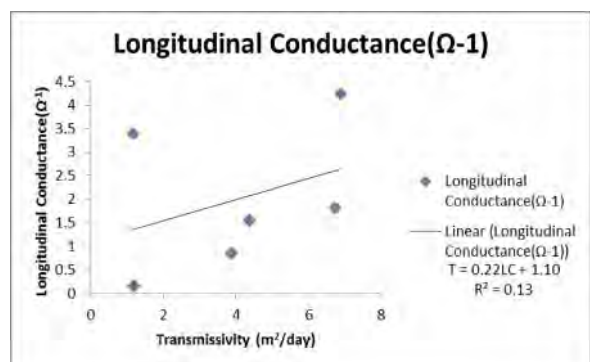
Figure 10: Longitudinal Conductance Against Transmissivity of the Aquifer
