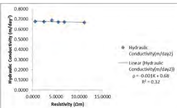
Figure 6: Hydraulic Conductivity Against Resistivity of the Aquifer
