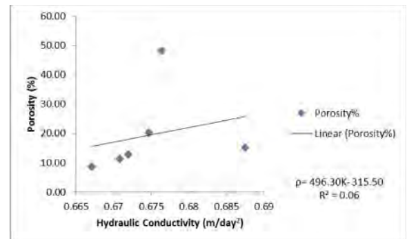
Figure 8: Porosity Against Hydraulic Conductivity of the Aquifer
