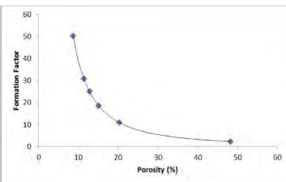
Figure 7: Formation Factor Against Porosity of the Aquifer
