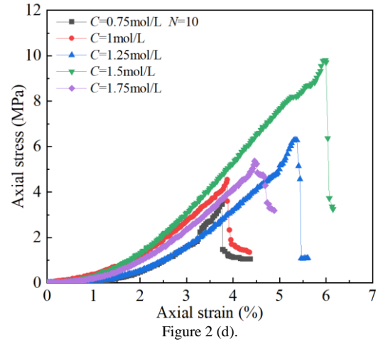
Figure 2. Unconfined compressive strength test results, (a). Stress-strain curves of UCS tests ( N=4 ; C=0.75/1/1.25/1.5/1.75 mol/L), (b). Stress-strain curves of UCS tests, ( N=6 ; C=0.75/1/1.25/1.5/1.75 mol/L), (c). Stress-strain curves of UCS tests ( N=8 ; C=0.75/1/1.25/1.5/1.75 mol/L), (d). Stress-strain curves of UCS tests, ( N=10 ; C=0.75/1/1.25/1.5/1.75 mol/L).
