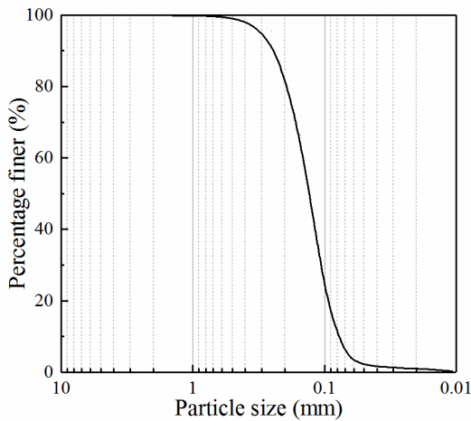
Figure 1. Grading curve of river silt.
