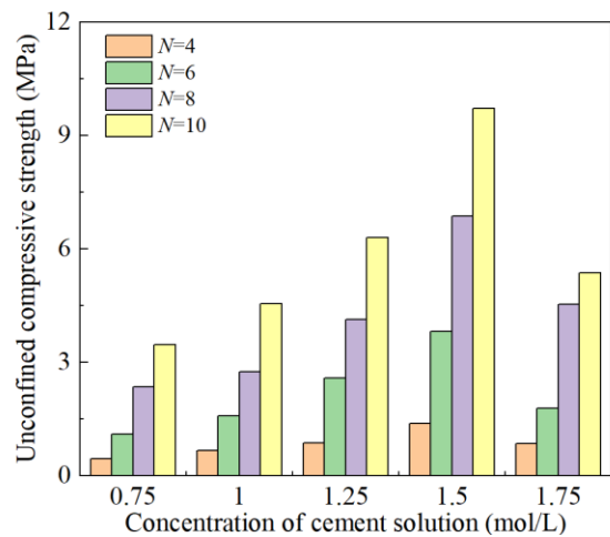
Figure 3. Unconfined compressive strength of soil samples with different concentration of cement solution and grouting times.
